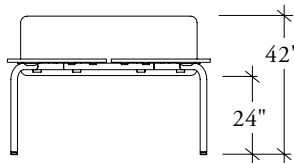
Slim Modesty Height (24" from the floor)
