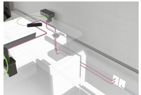
Cable routing through backs of storage
